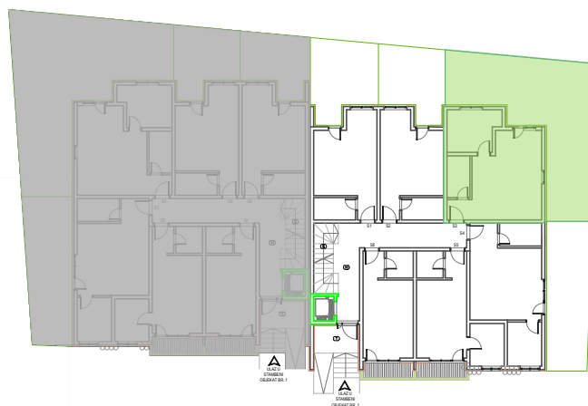
Pozicija stana 03 u zgradi /Position of apartment 03 in the building
