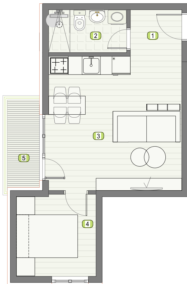
Osnova stana 15 /Top view of the apartment 15
